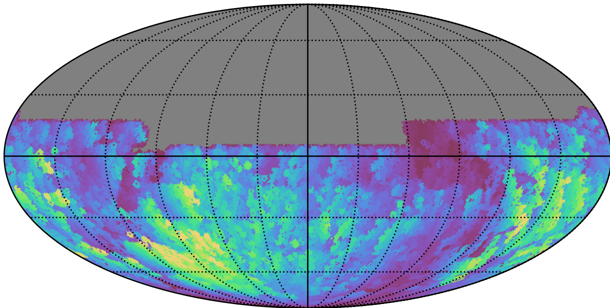
weather_cloudso12v3.4_10yrs All sky u band: Max normairmass
