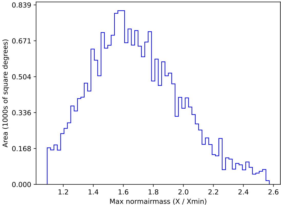
weather_cloudso12v3.4_10yrs All sky u band: Max normairmass
