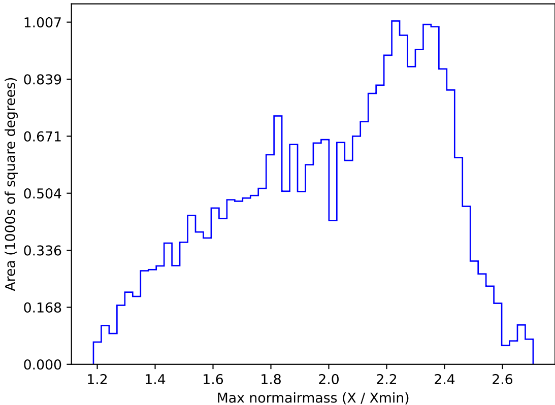
weather_cloudso12v3.4_10yrs All sky r band: Max normairmass
