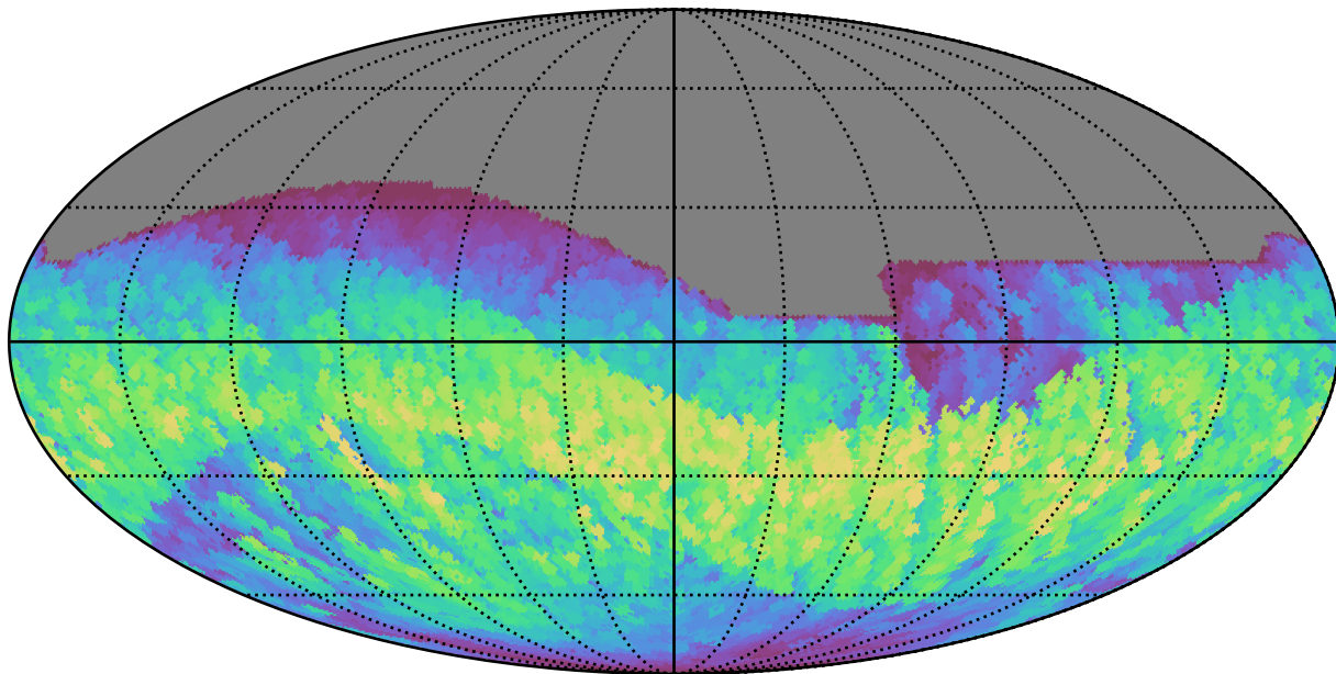
weather_cloudso12v3.4_10yrs All sky i band: Max normairmass
