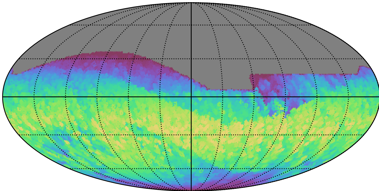
weather_cloudso12v3.4_10yrs All sky all bands: Max normairmass
