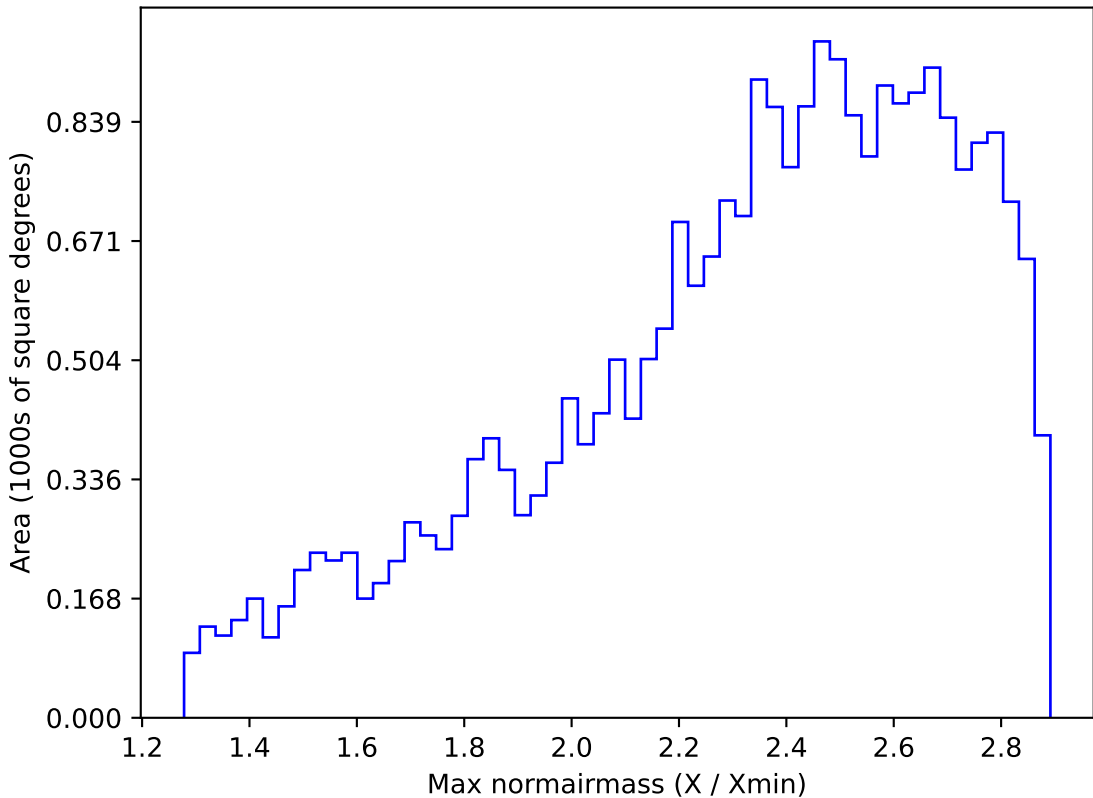
weather_cloudso12v3.4_10yrs All sky all bands: Max normairmass
