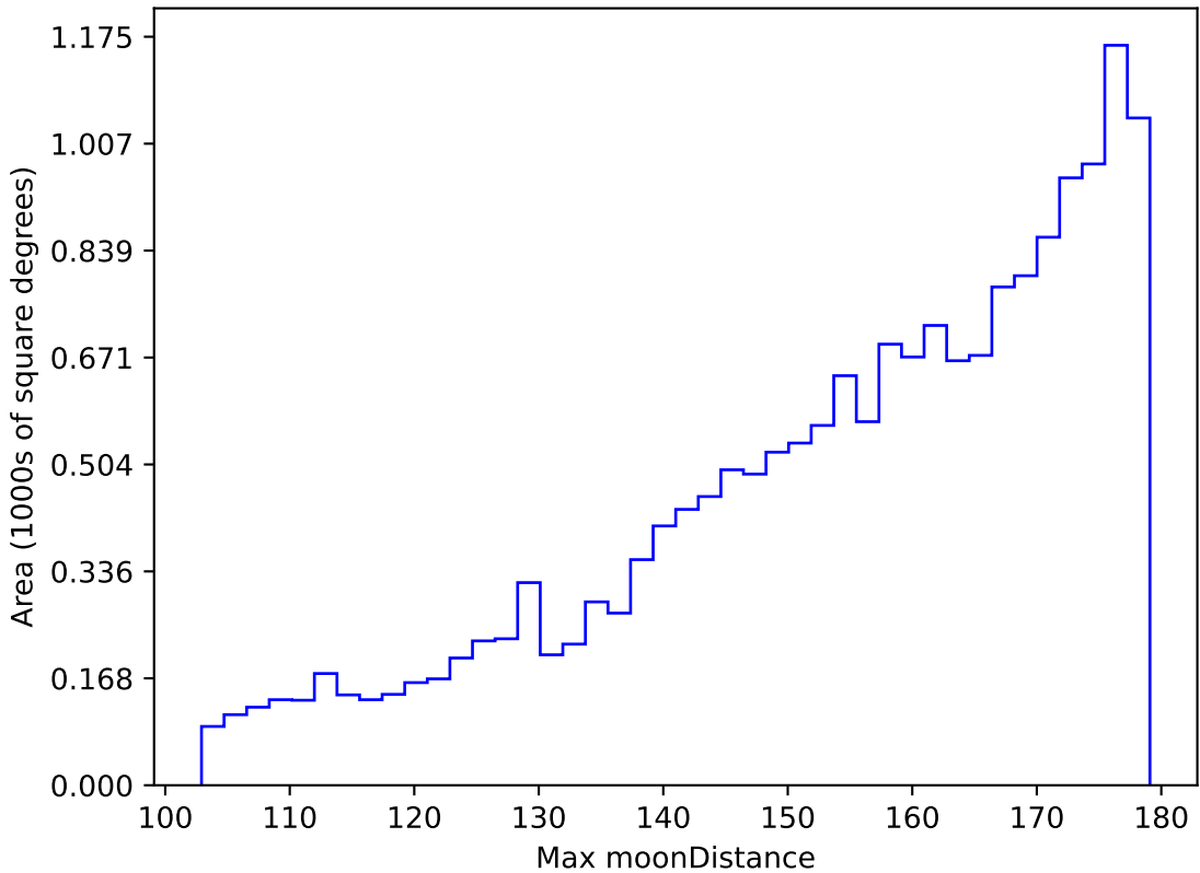
weather_cloudso12v3.4_10yrs WFD z band: Max moonDistance
