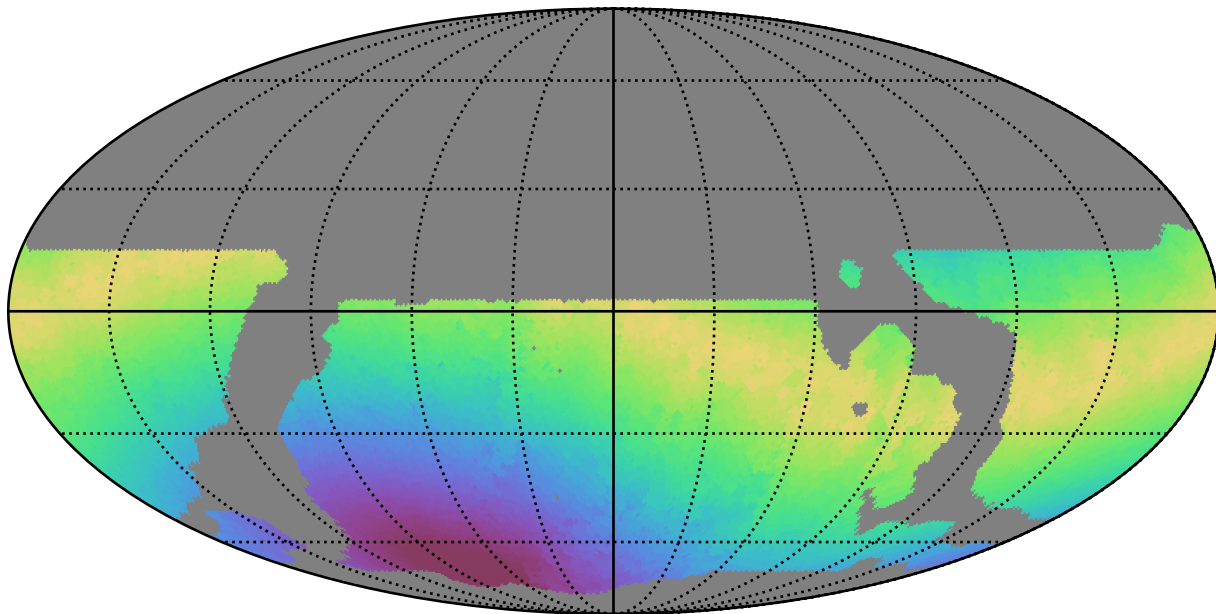
weather_cloudso12v3.4_10yrs WFD u band: Max moonDistance
