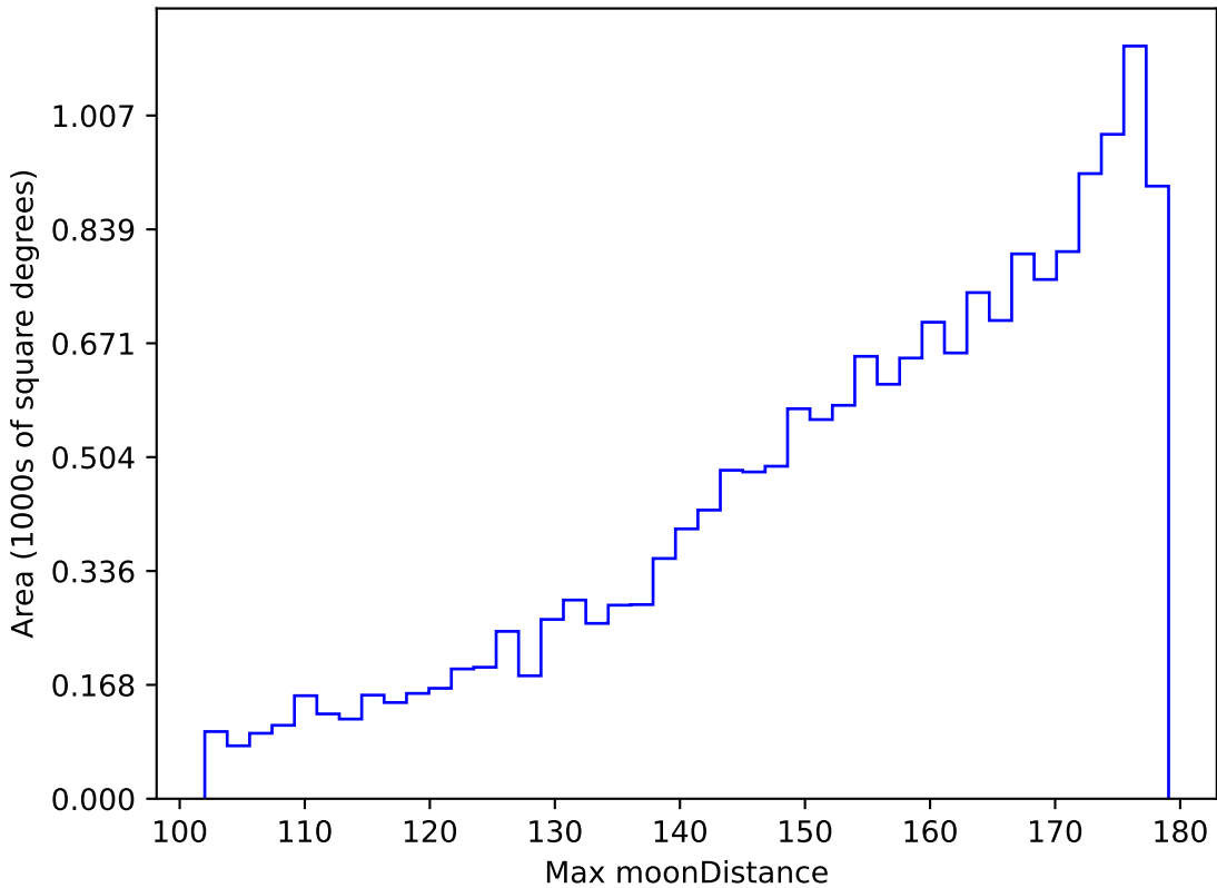
weather_cloudso12v3.4_10yrs WFD u band: Max moonDistance
