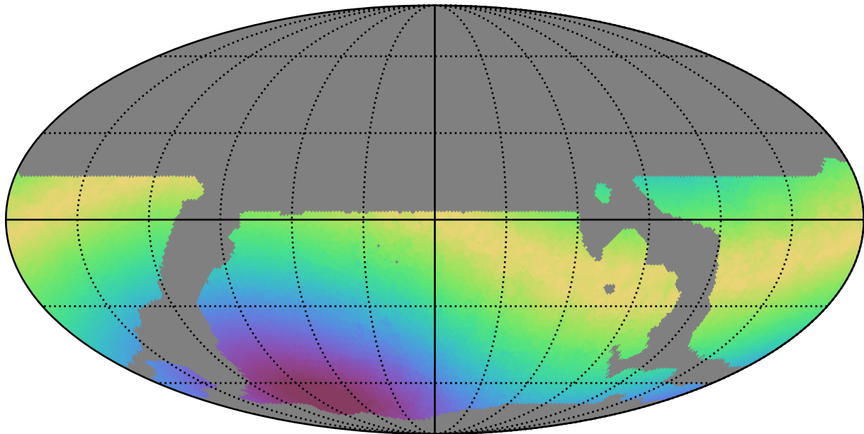
weather_cloudso12v3.4_10yrs WFD r band: Max moonDistance
