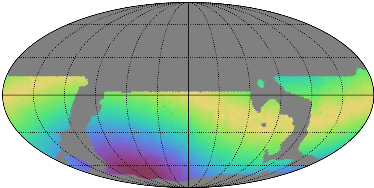
weather_cloudso12v3.4_10yrs WFD i band: Max moonDistance
