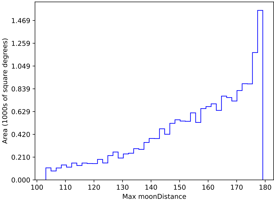
weather_cloudso12v3.4_10yrs WFD i band: Max moonDistance
