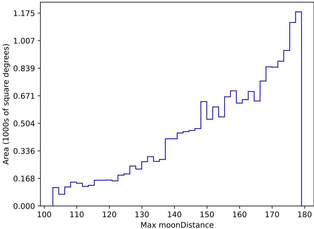
weather_cloudso12v3.4_10yrs WFD g band: Max moonDistance
