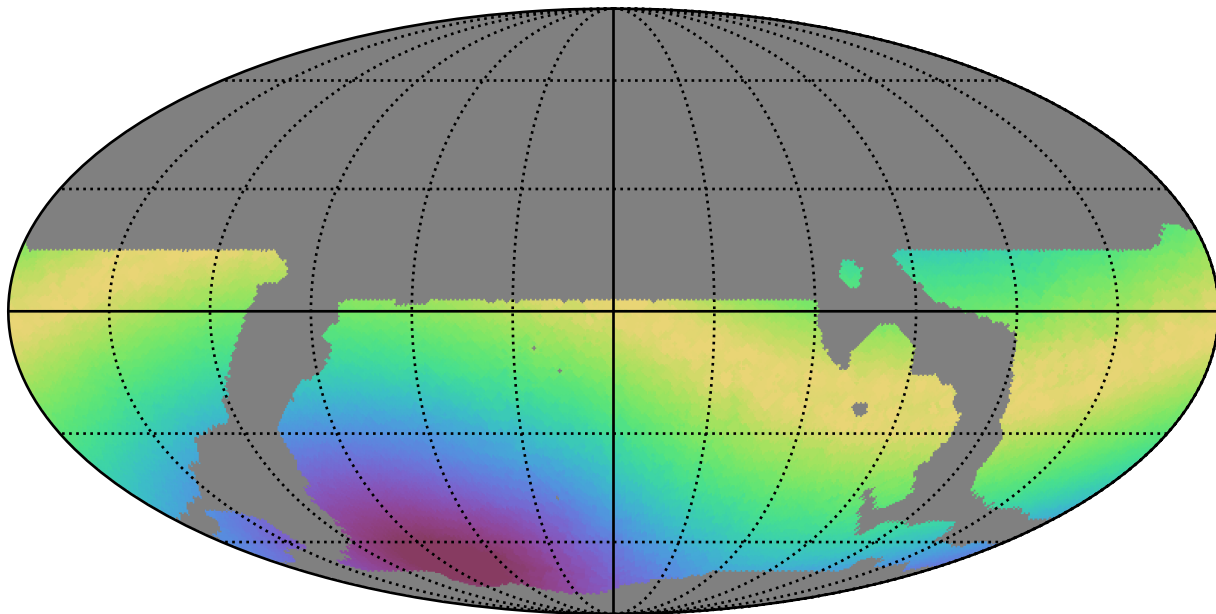
weather_cloudso12v3.4_10yrs WFD all bands: Max moonDistance
