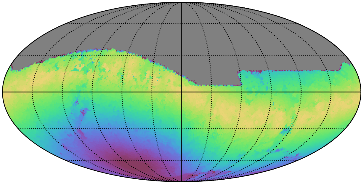
weather_cloudso12v3.4_10yrs All sky z band: Max moonDistance
