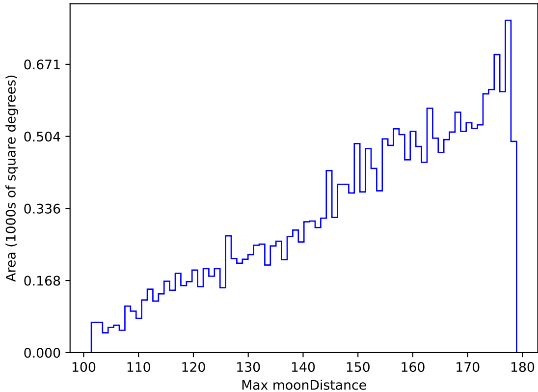
weather_cloudso12v3.4_10yrs All sky u band: Max moonDistance
