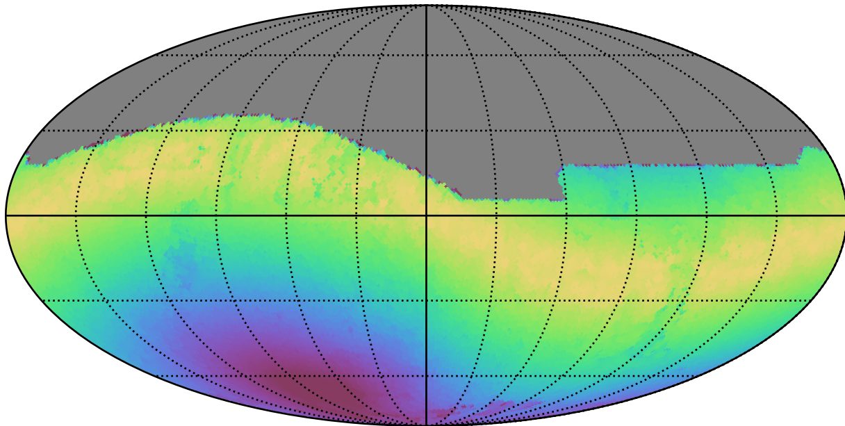
weather_cloudso12v3.4_10yrs All sky i band: Max moonDistance
