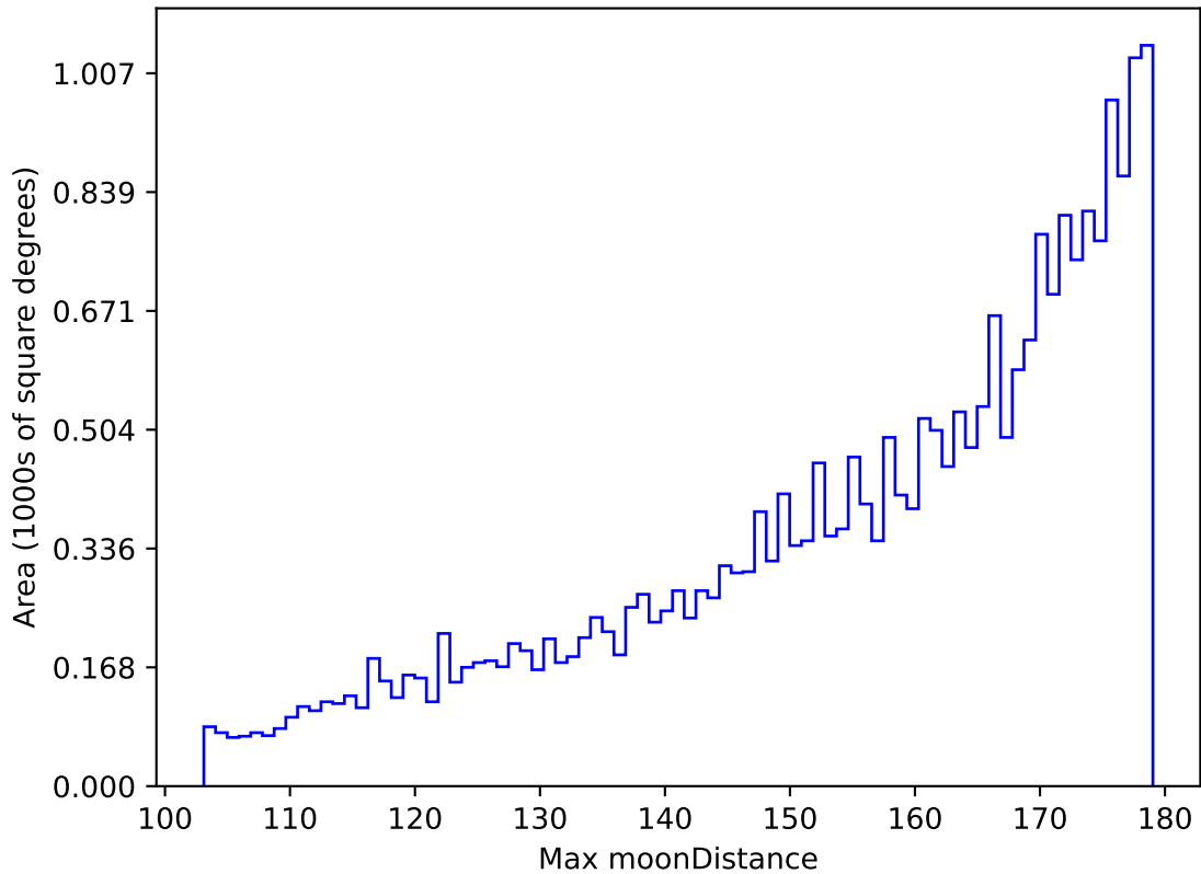
weather_cloudso12v3.4_10yrs All sky i band: Max moonDistance
