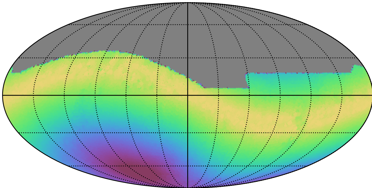
weather_cloudso12v3.4_10yrs All sky all bands: Max moonDistance
