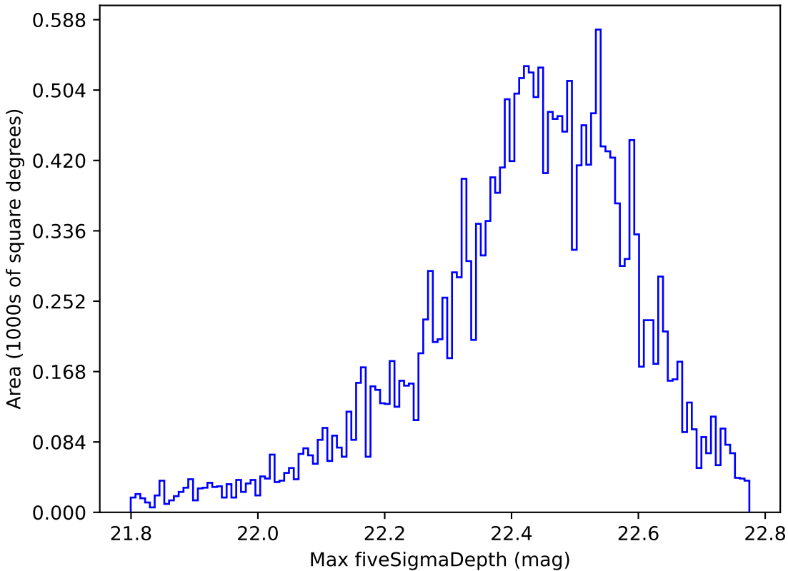
weather_cloudso12v3.4_10yrs Yr 1 y band: Max fiveSigmaDepth
