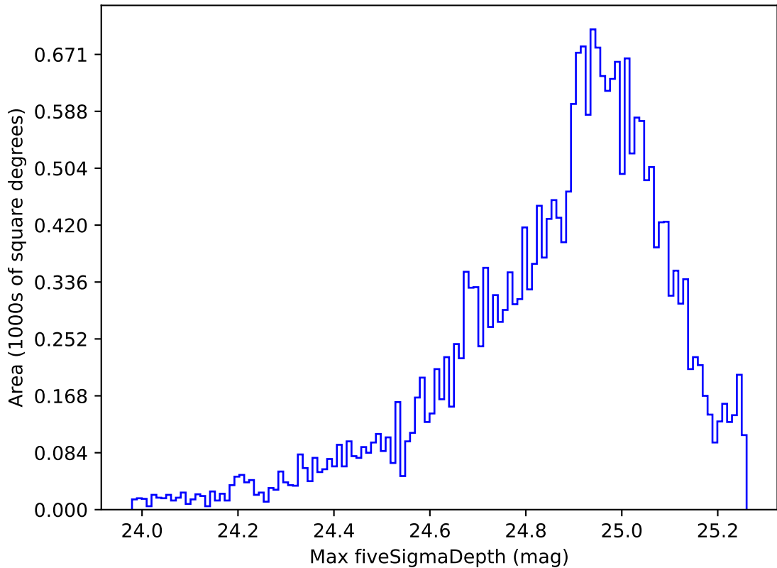
weather_cloudso12v3.4_10yrs Yr 1 g band: Max fiveSigmaDepth
