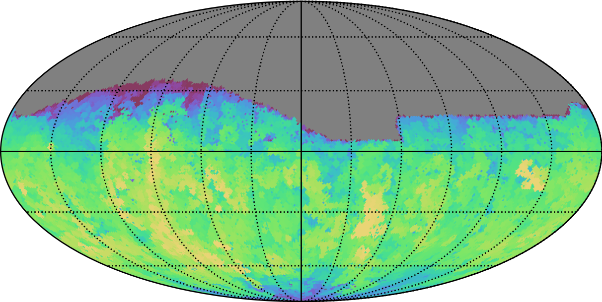
weather_cloudso12v3.4_10yrs Yr 1 all bands: Max fiveSigmaDepth
