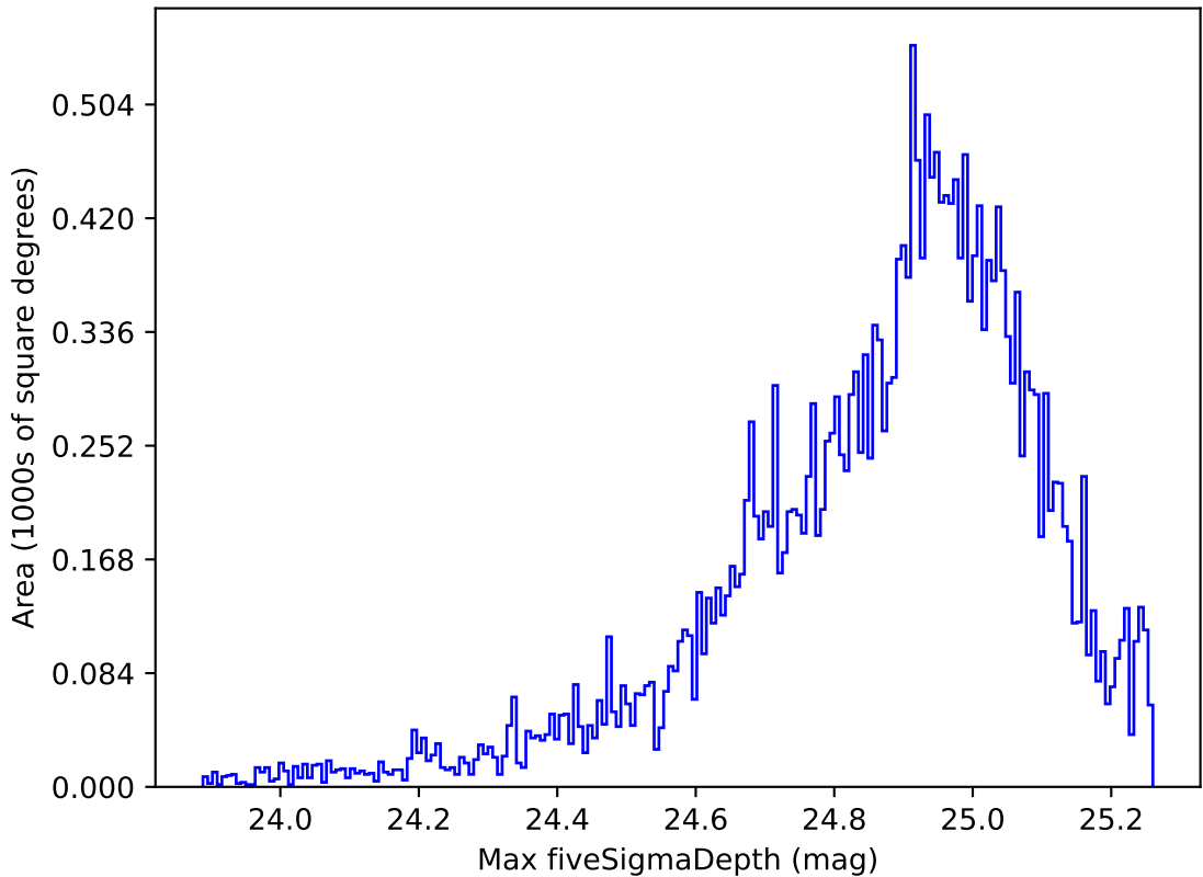
weather_cloudso12v3.4_10yrs Yr 1 all bands: Max fiveSigmaDepth
