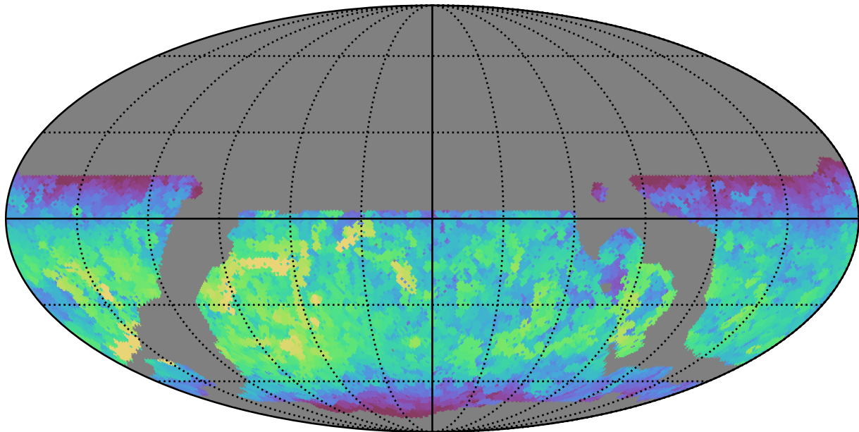
weather_cloudso12v3.4_10yrs WFD y band: Max fiveSigmaDepth
