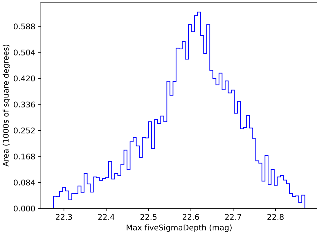
weather_cloudso12v3.4_10yrs WFD y band: Max fiveSigmaDepth
