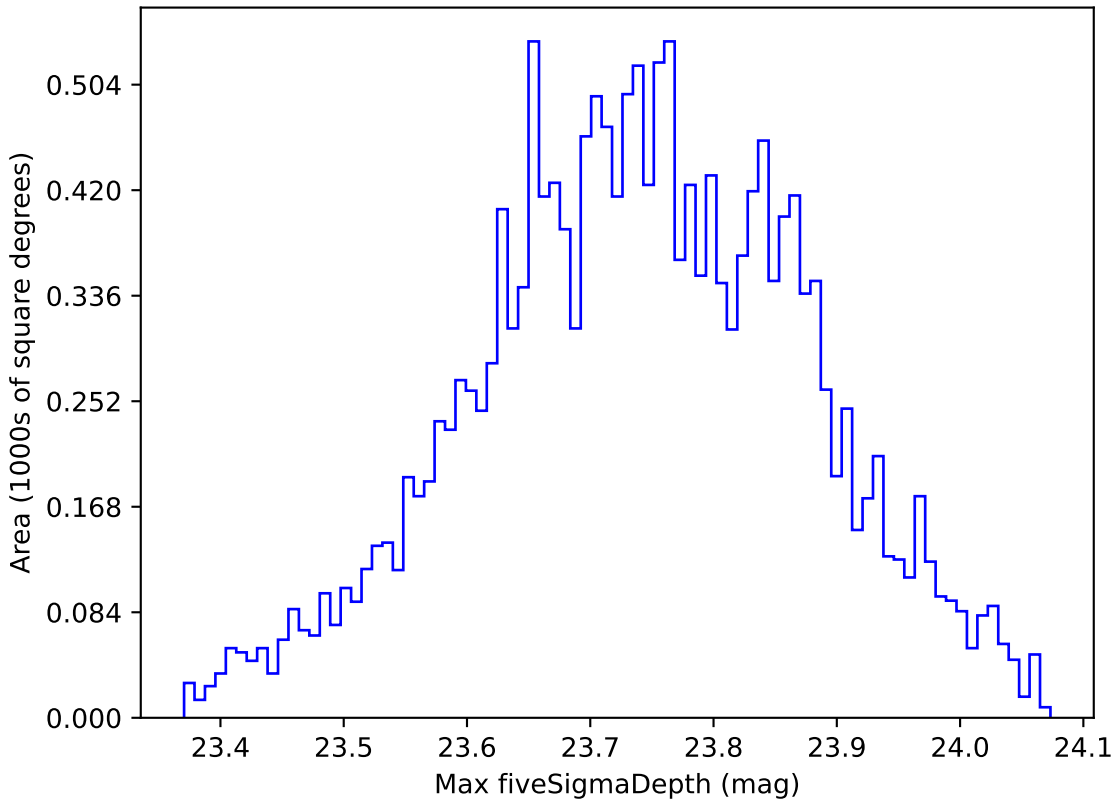
weather_cloudso12v3.4_10yrs WFD u band: Max fiveSigmaDepth
