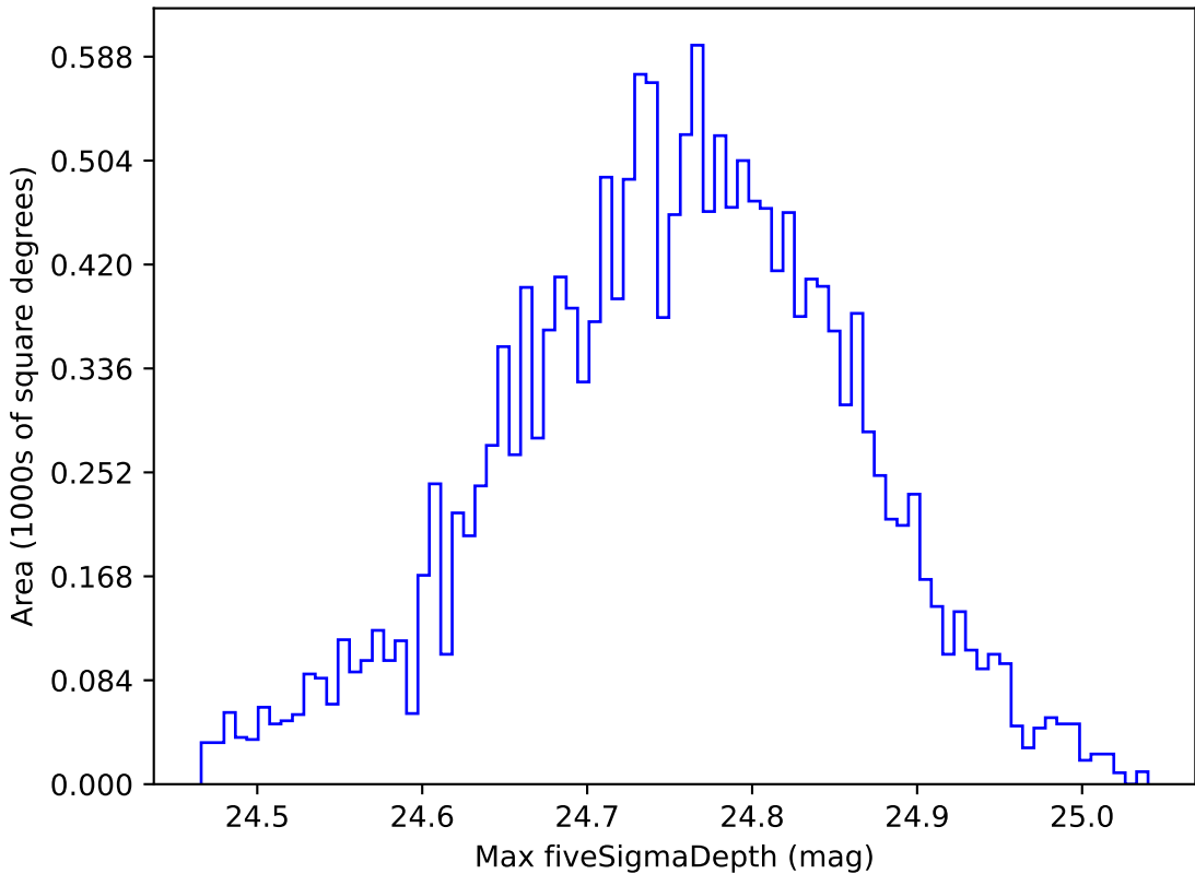
weather_cloudso12v3.4_10yrs WFD r band: Max fiveSigmaDepth
