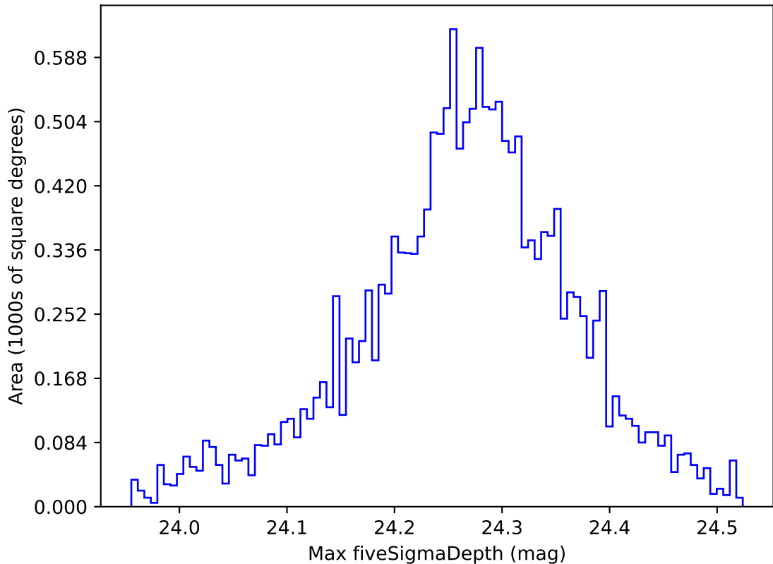
weather_cloudso12v3.4_10yrs WFD i band: Max fiveSigmaDepth
