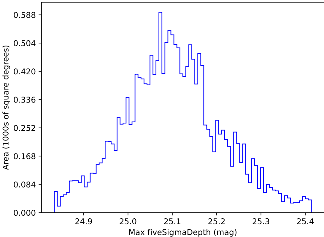
weather_cloudso12v3.4_10yrs WFD g band: Max fiveSigmaDepth
