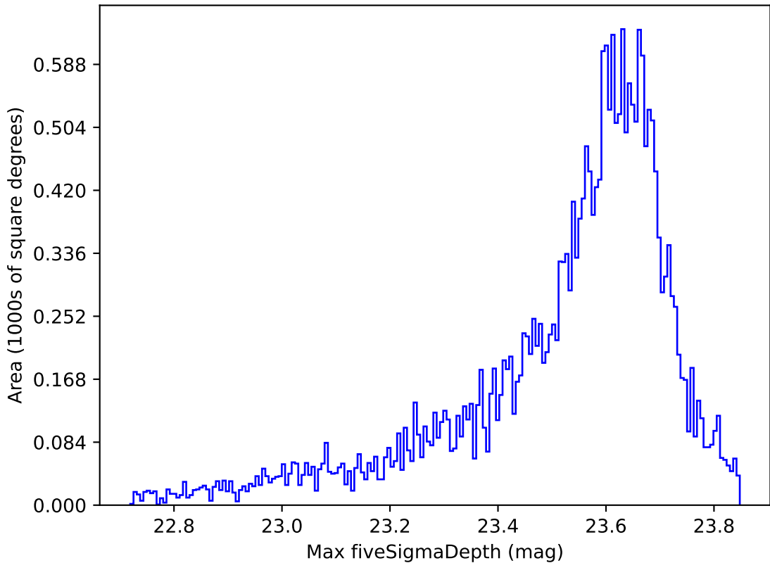
weather_cloudso12v3.4_10yrs All sky z band: Max fiveSigmaDepth
