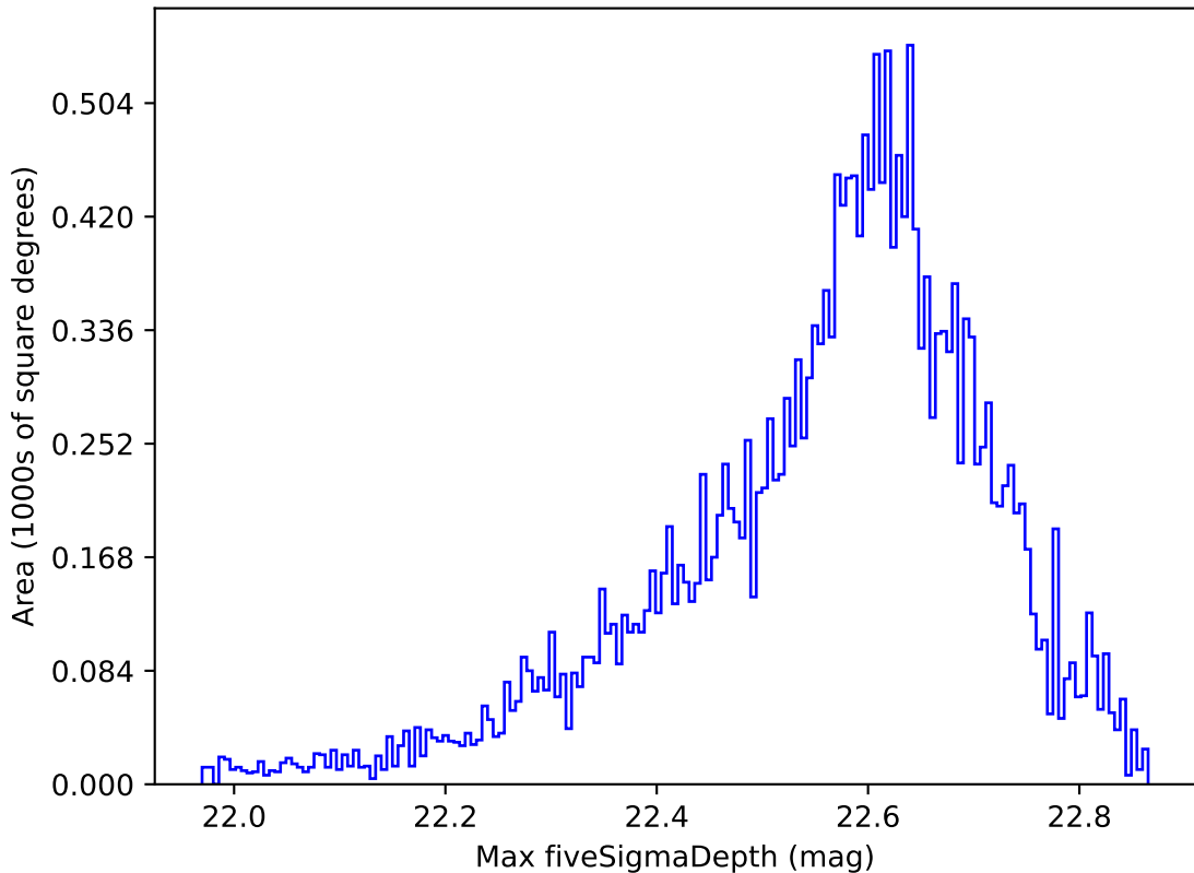
weather_cloudso12v3.4_10yrs All sky y band: Max fiveSigmaDepth
