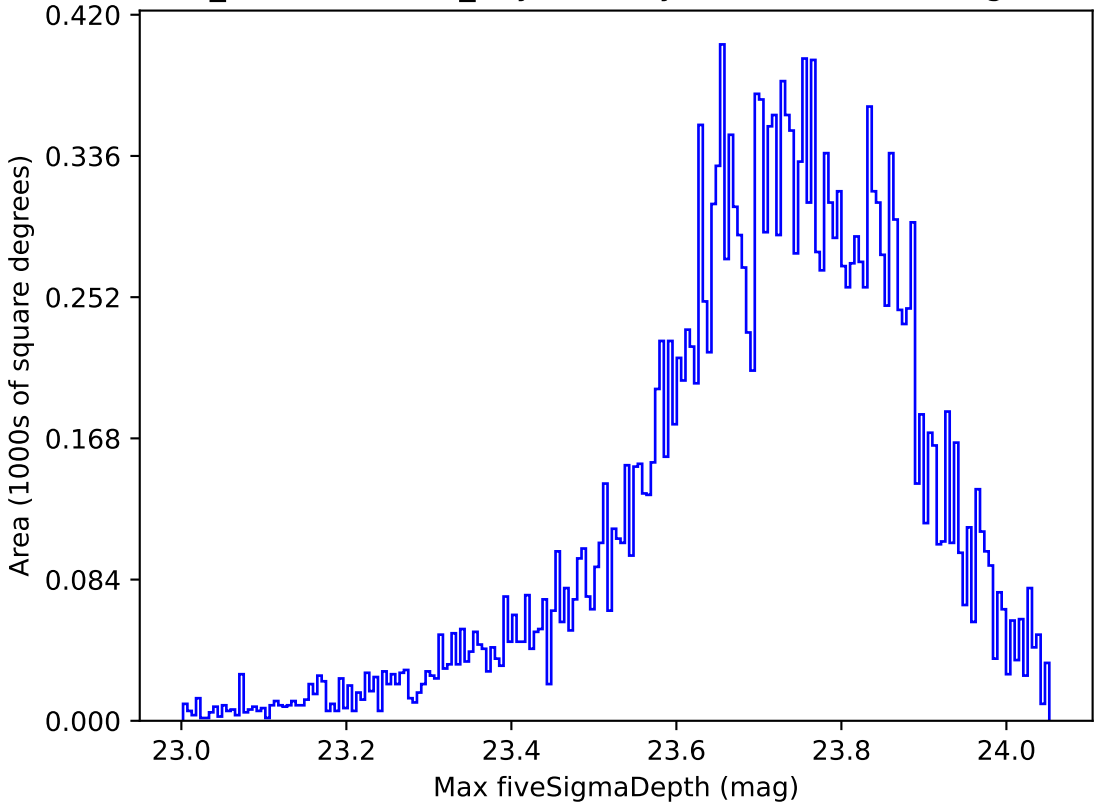
weather_cloudso12v3.4_10yrs All sky u band: Max fiveSigmaDepth
