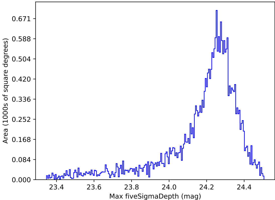
weather_cloudso12v3.4_10yrs All sky i band: Max fiveSigmaDepth
