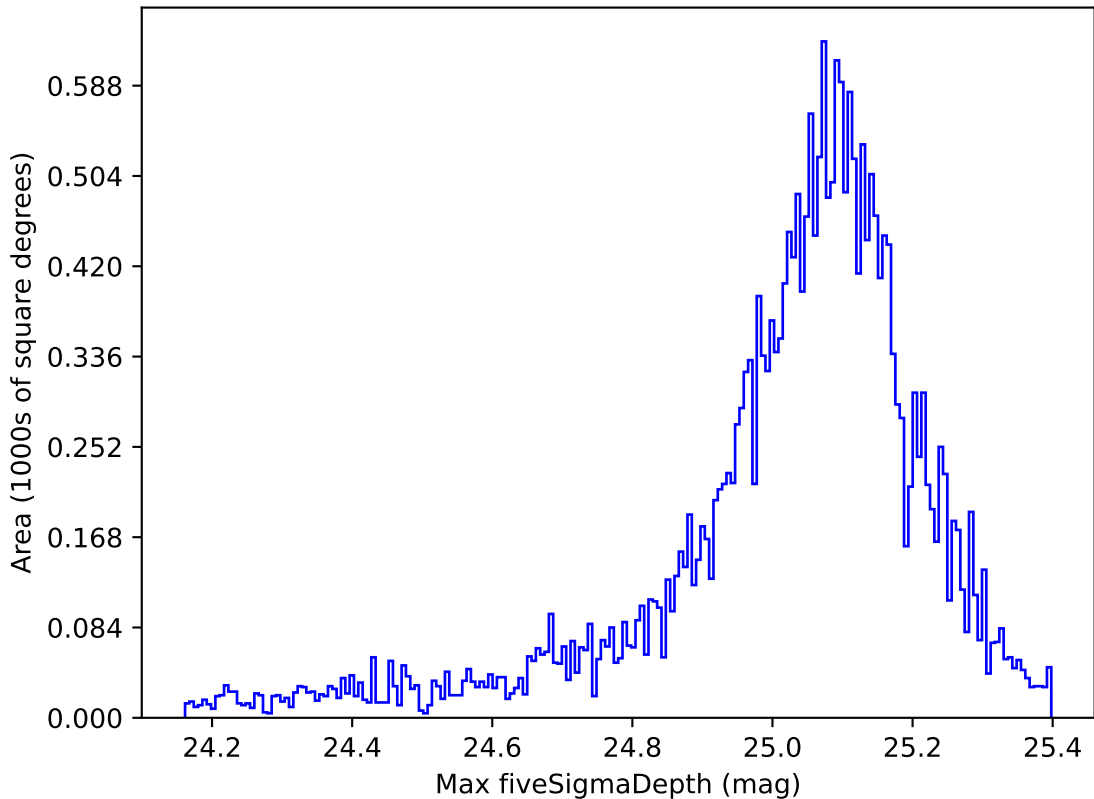
weather_cloudso12v3.4_10yrs All sky g band: Max fiveSigmaDepth
