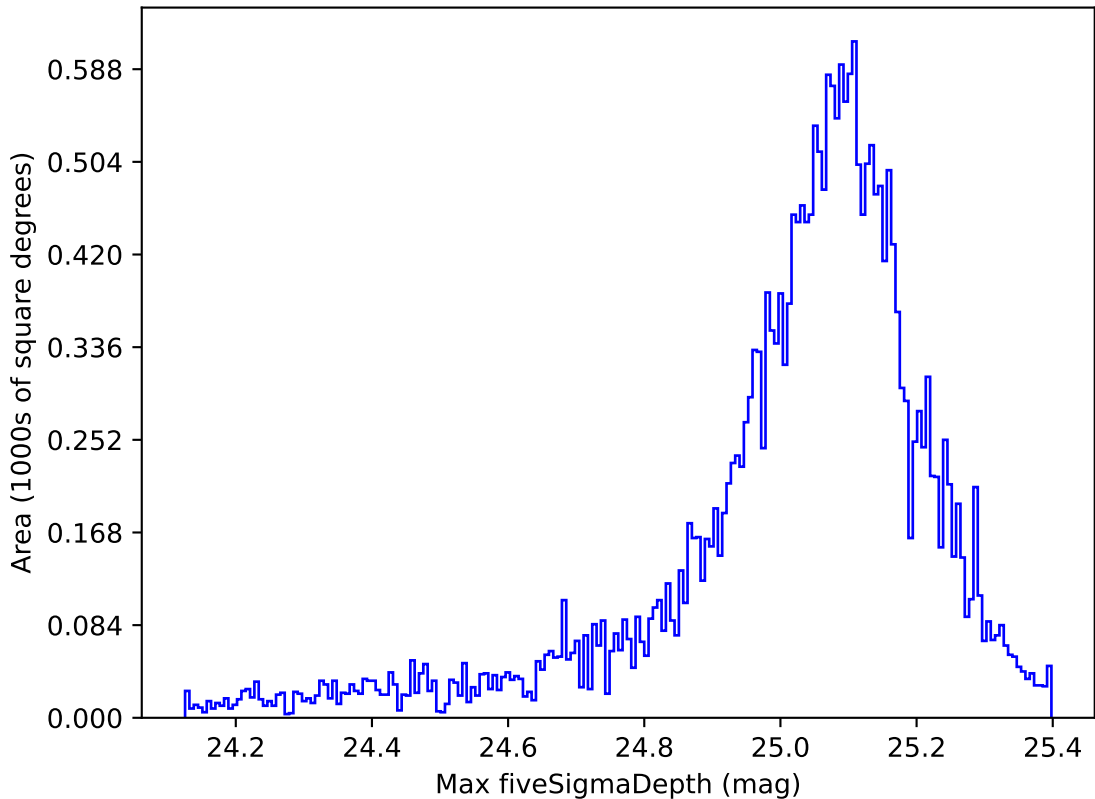
weather_cloudso12v3.4_10yrs All sky all bands: Max fiveSigmaDepth
