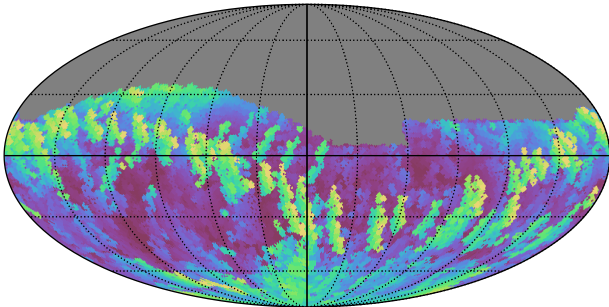
weather_cloudso12v3.4_10yrs Yr 1 z band: Max airmass
