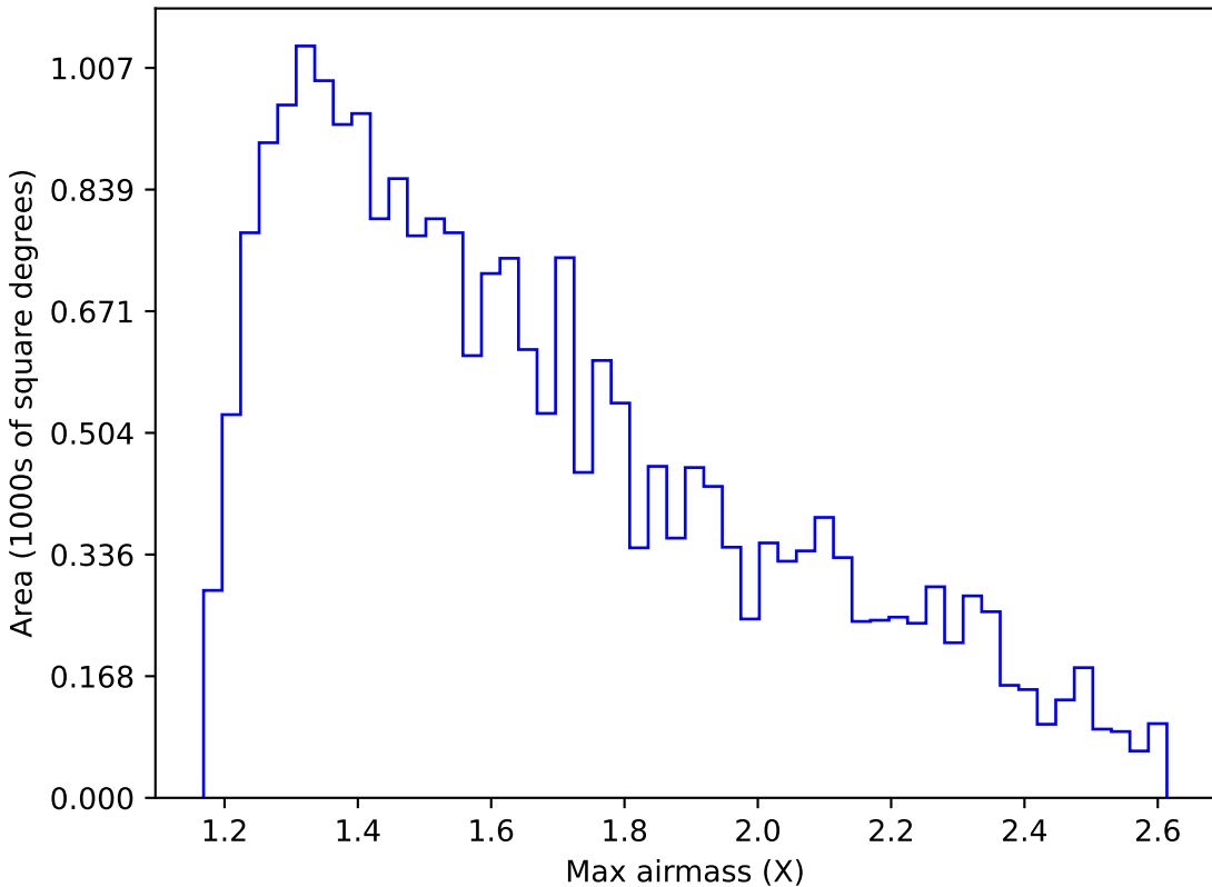
weather_cloudso12v3.4_10yrs Yr 1 y band: Max airmass
