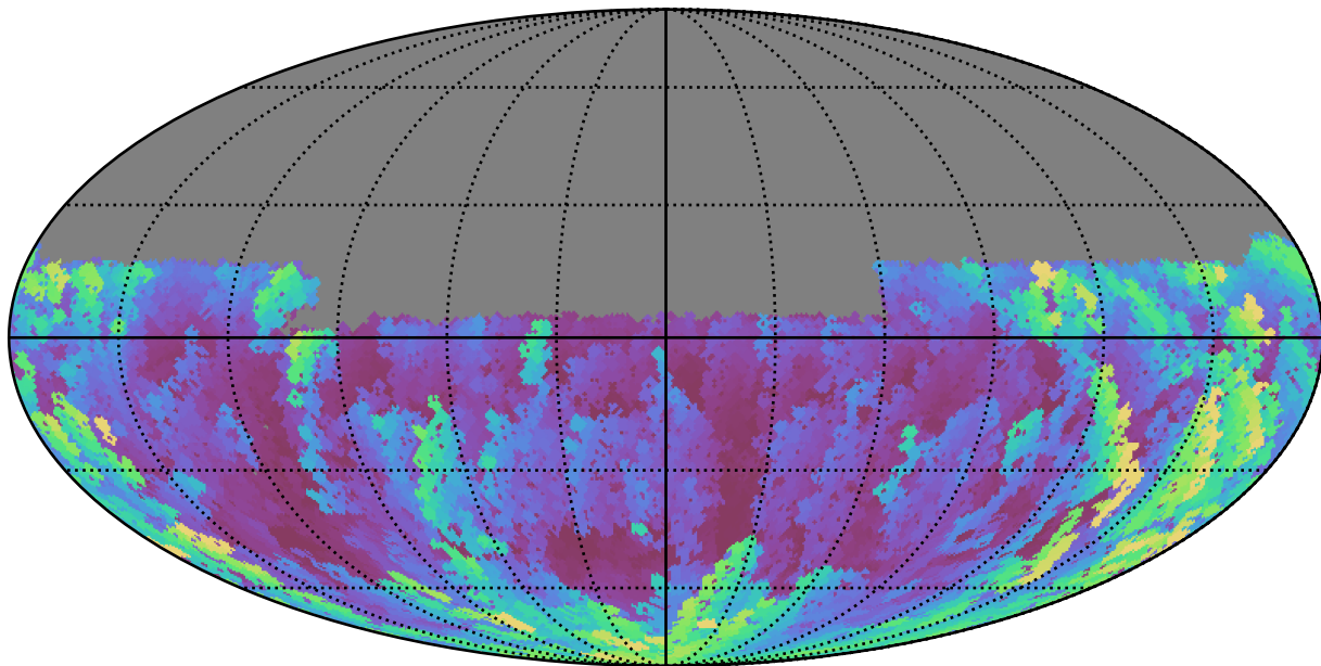
weather_cloudso12v3.4_10yrs Yr 1 u band: Max airmass
