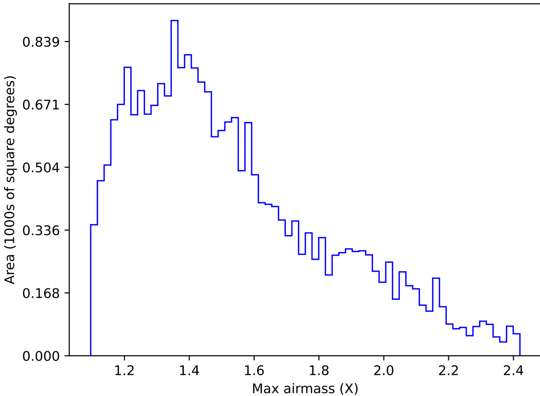
weather_cloudso12v3.4_10yrs Yr 1 u band: Max airmass
