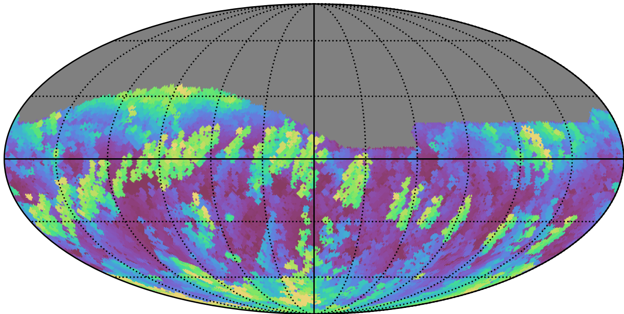
weather_cloudso12v3.4_10yrs Yr 1 r band: Max airmass
