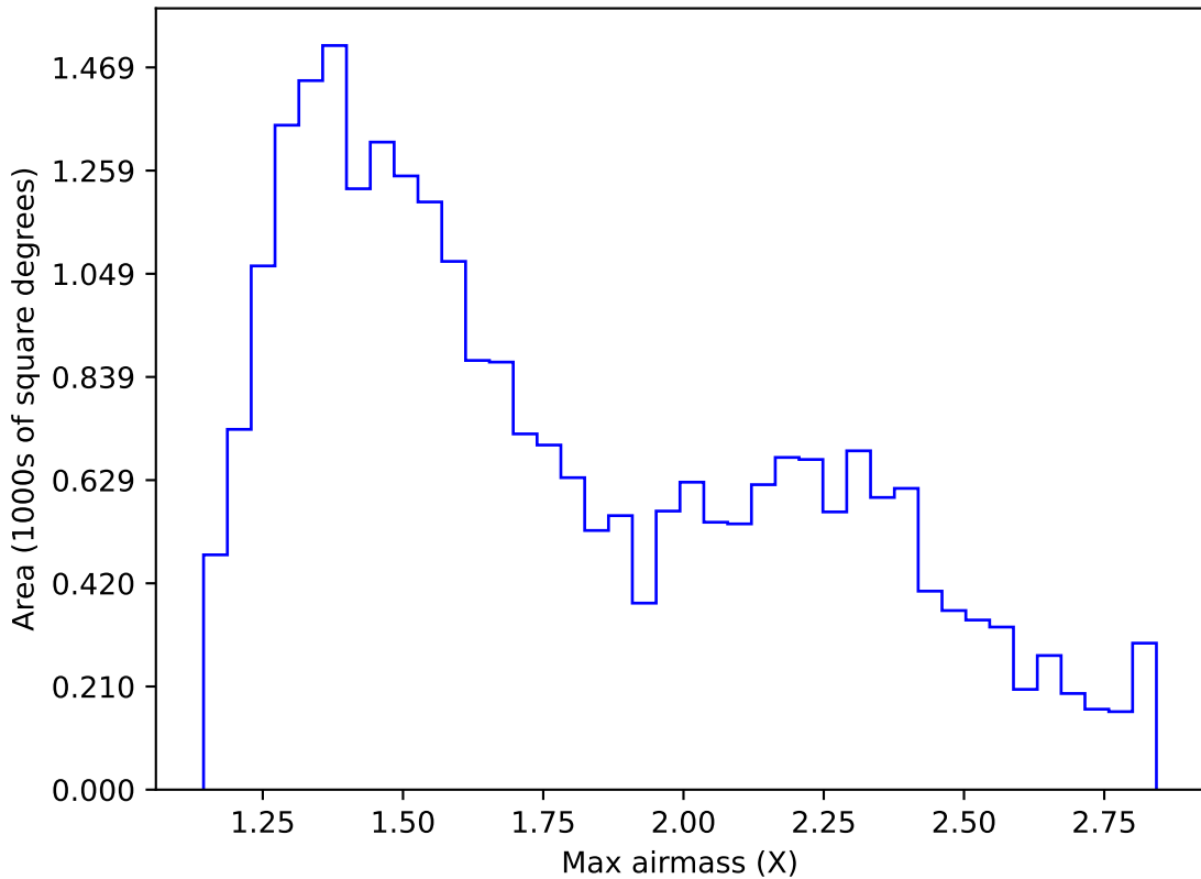
weather_cloudso12v3.4_10yrs Yr 1 i band: Max airmass
