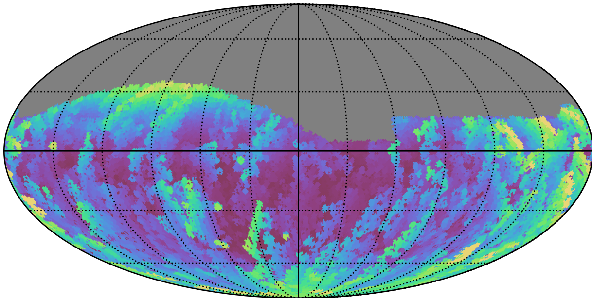
weather_cloudso12v3.4_10yrs Yr 1 g band: Max airmass
