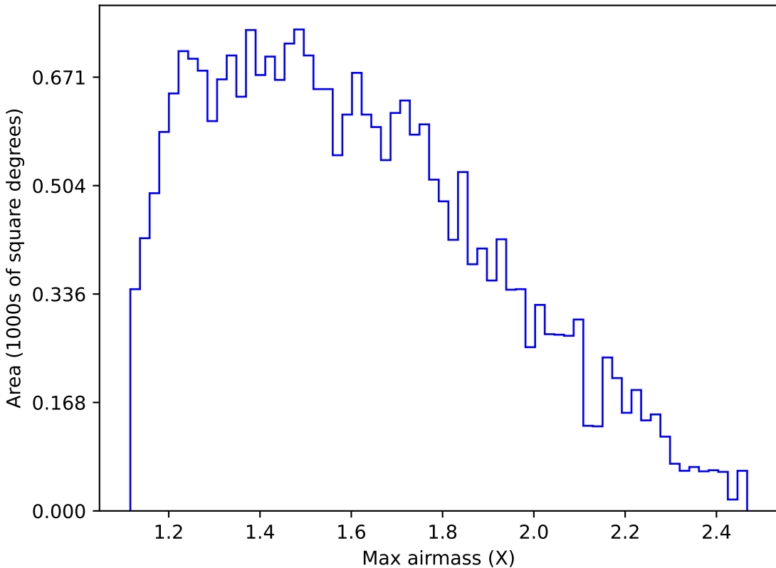
weather_cloudso12v3.4_10yrs Yr 1 g band: Max airmass
