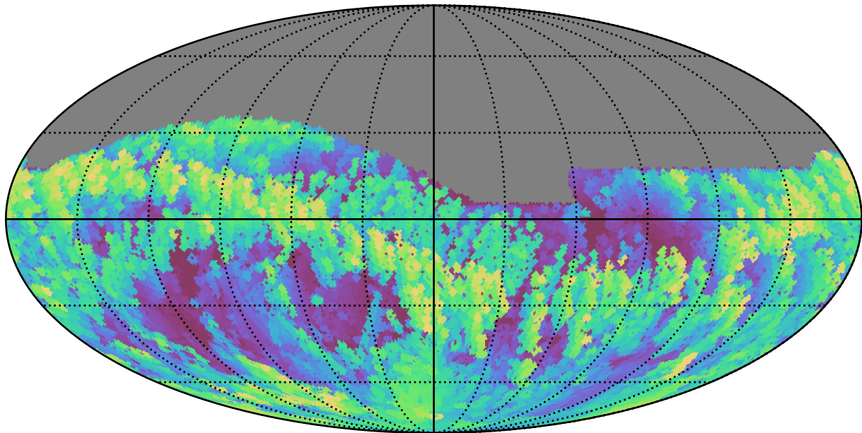
weather_cloudso12v3.4_10yrs Yr 1 all bands: Max airmass
