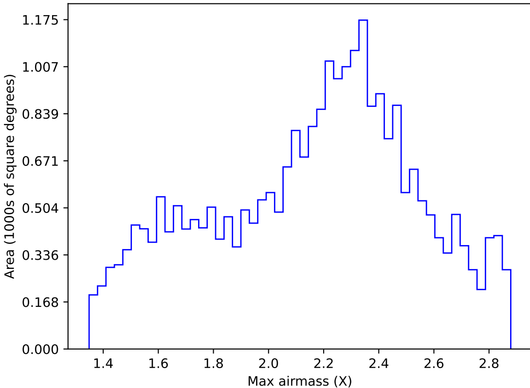
weather_cloudso12v3.4_10yrs Yr 1 all bands: Max airmass
