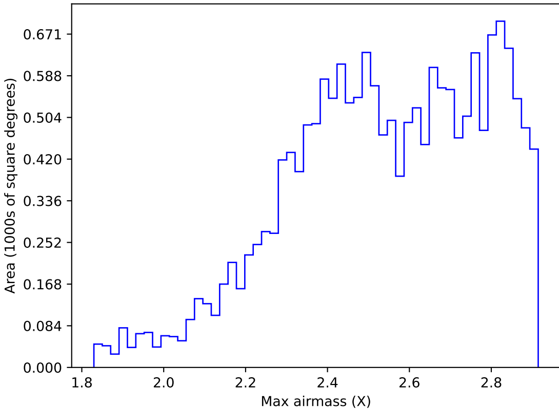
weather_cloudso12v3.4_10yrs WFD z band: Max airmass
