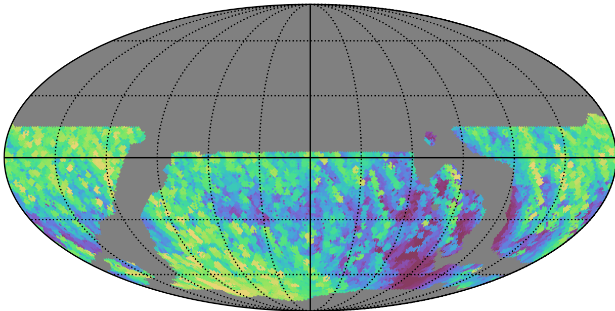
weather_cloudso12v3.4_10yrs WFD y band: Max airmass
