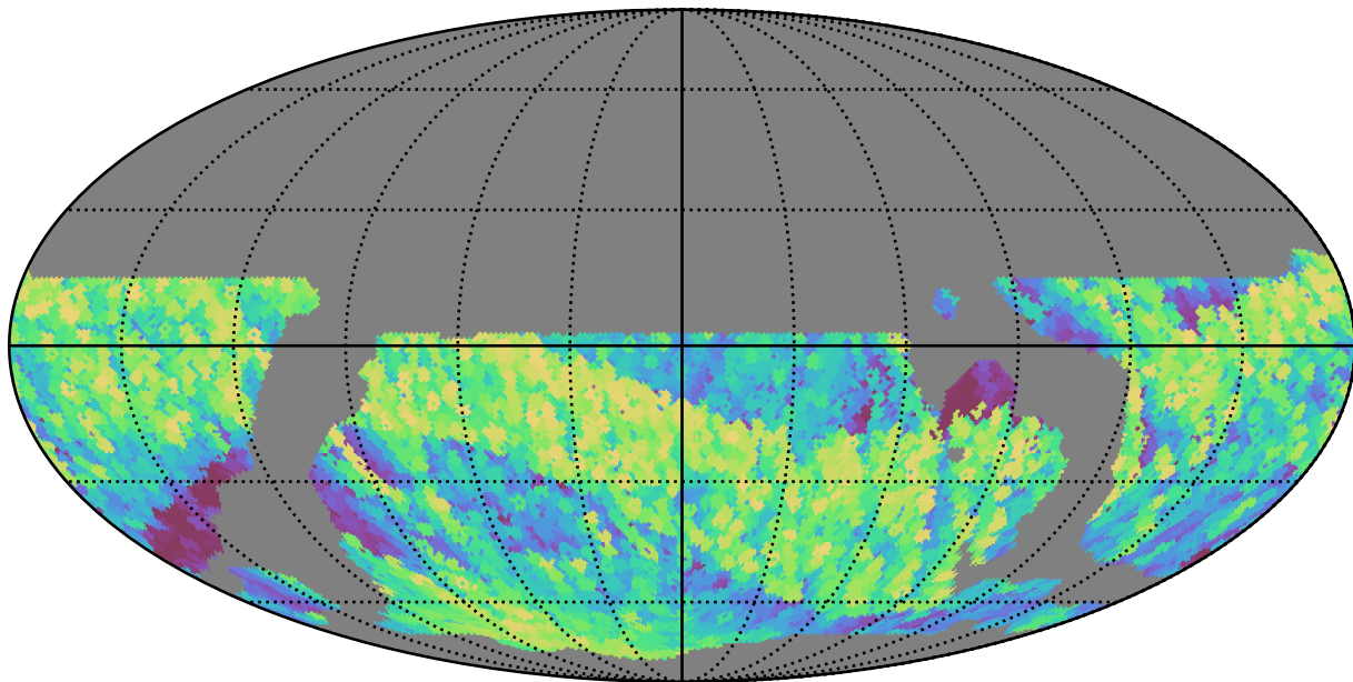
weather_cloudso12v3.4_10yrs WFD i band: Max airmass
