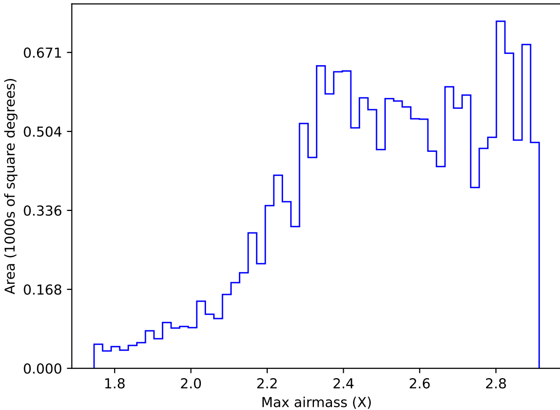
weather_cloudso12v3.4_10yrs WFD i band: Max airmass
