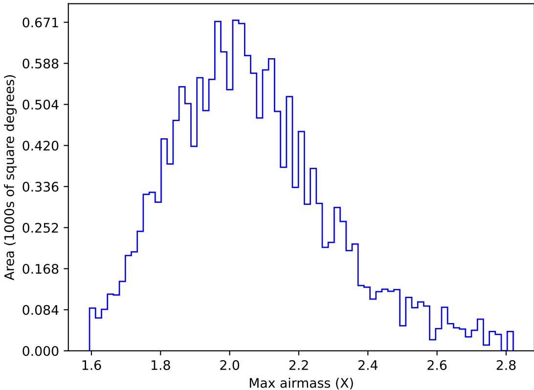
weather_cloudso12v3.4_10yrs WFD g band: Max airmass
